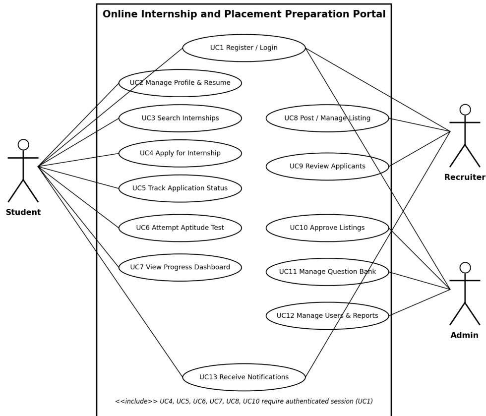
Figure 1: UML use case diagram of the Portal
